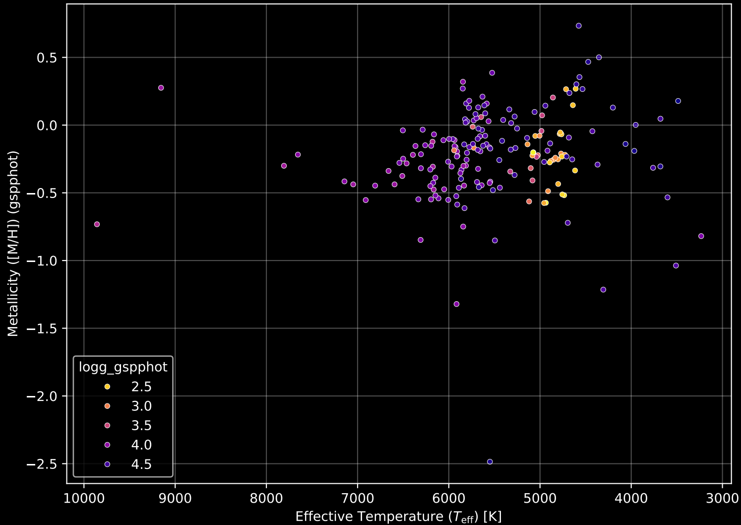
APOGEE DR17 Field: [062+43_MGA] Stellar Population Parameters (n= 186)
