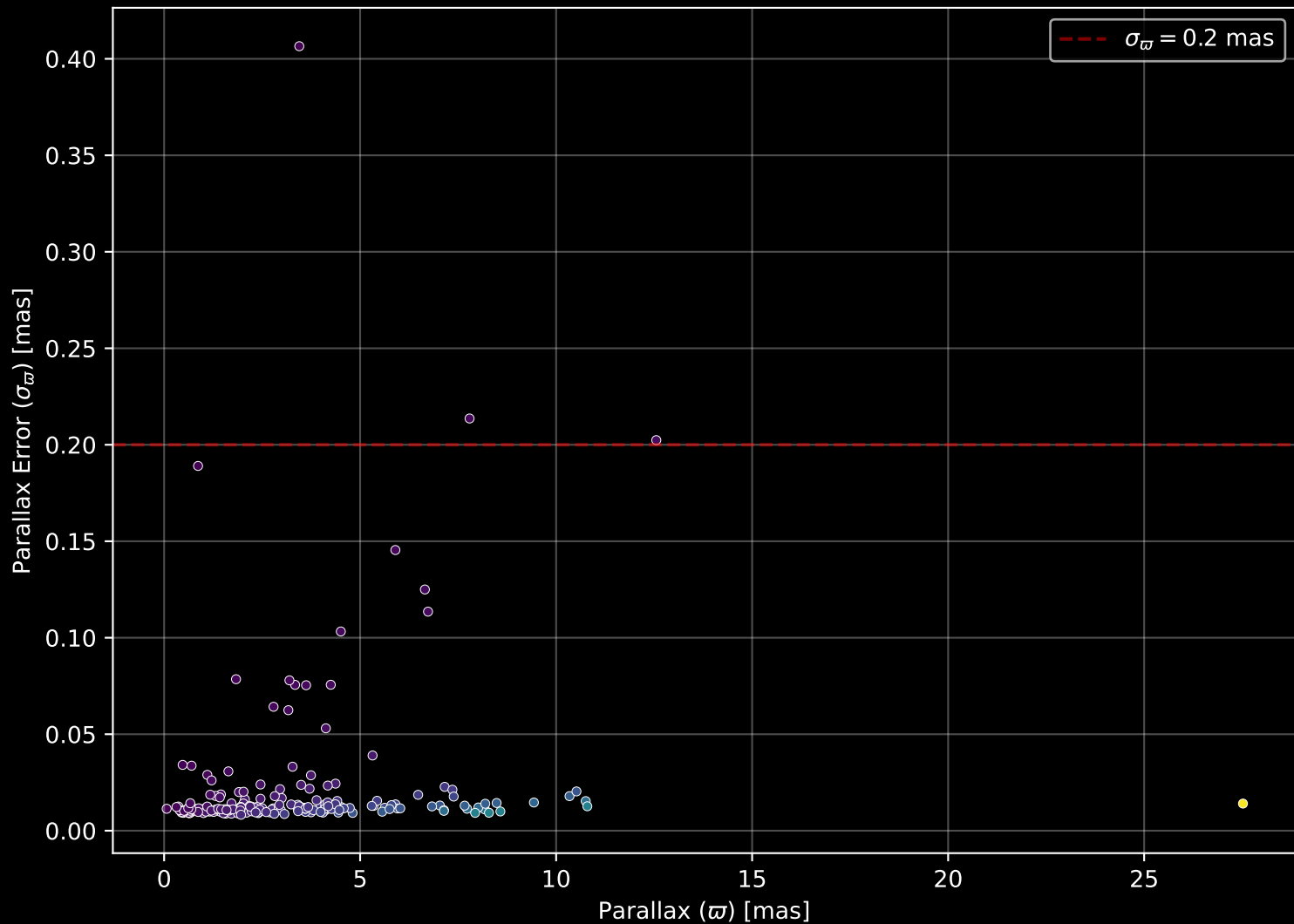
APOGEE DR17 Field: [062+43_MGA] Parallax Quality (n= 186)
