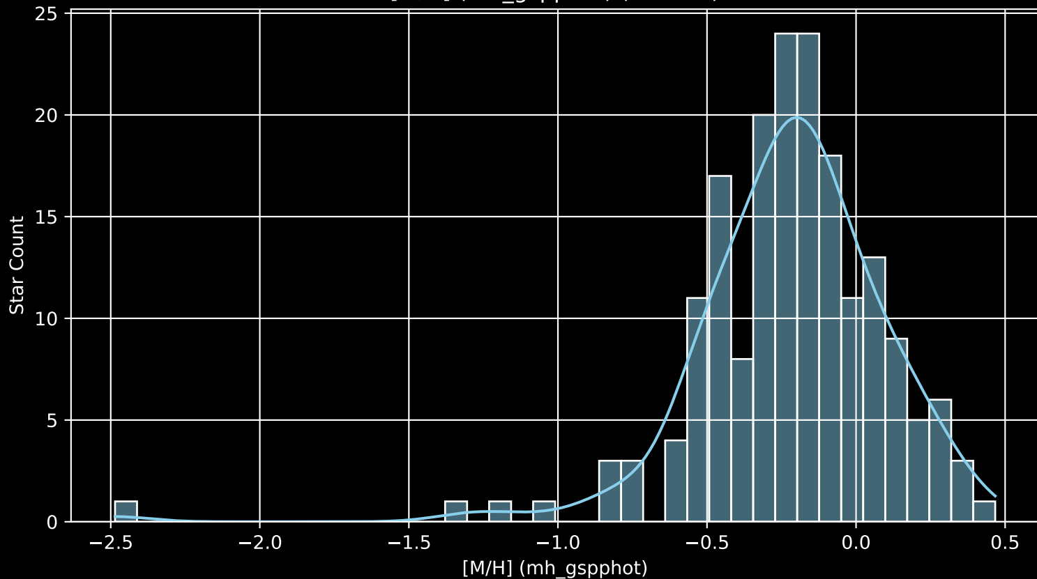
APOGEE DR17 Field: [062+43_MGA [M/H] (mh_gspphot) (n= 184)
