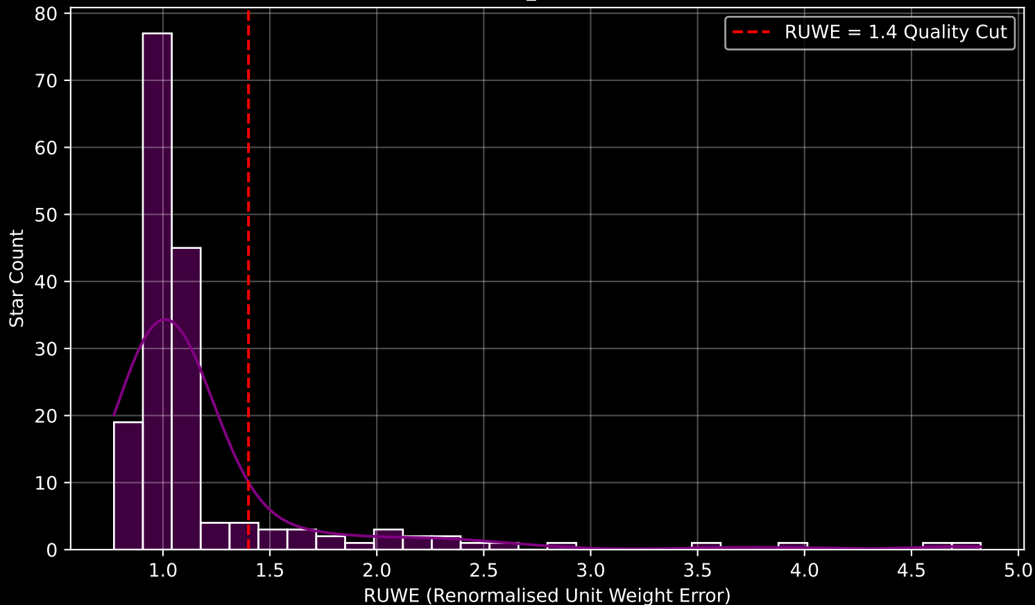
GAPOGEE DR17 Field [062+43_MGA] RUWE Distribution (n= 172)
