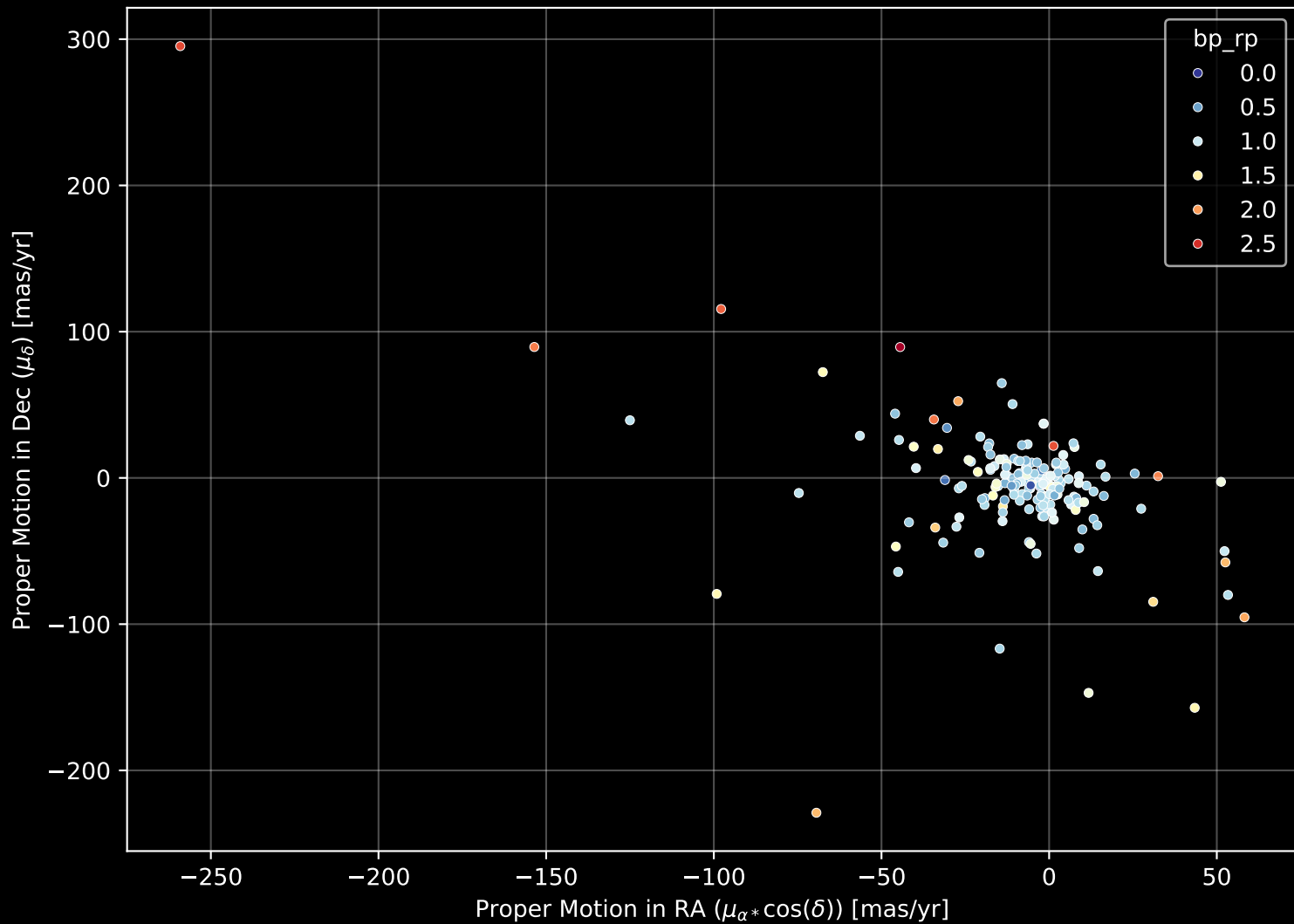
APOGEE DR17 Field: [062+43_MGA] Proper Motion Diagram (n= 186)
